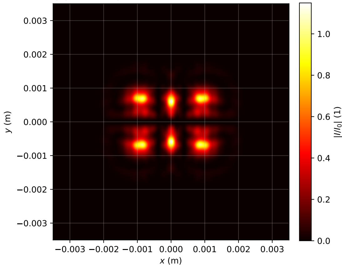
Intensity profile I(x, y, z = 1.353)/I_0 , P_{in}=7.0P_{cr} , artificial time
